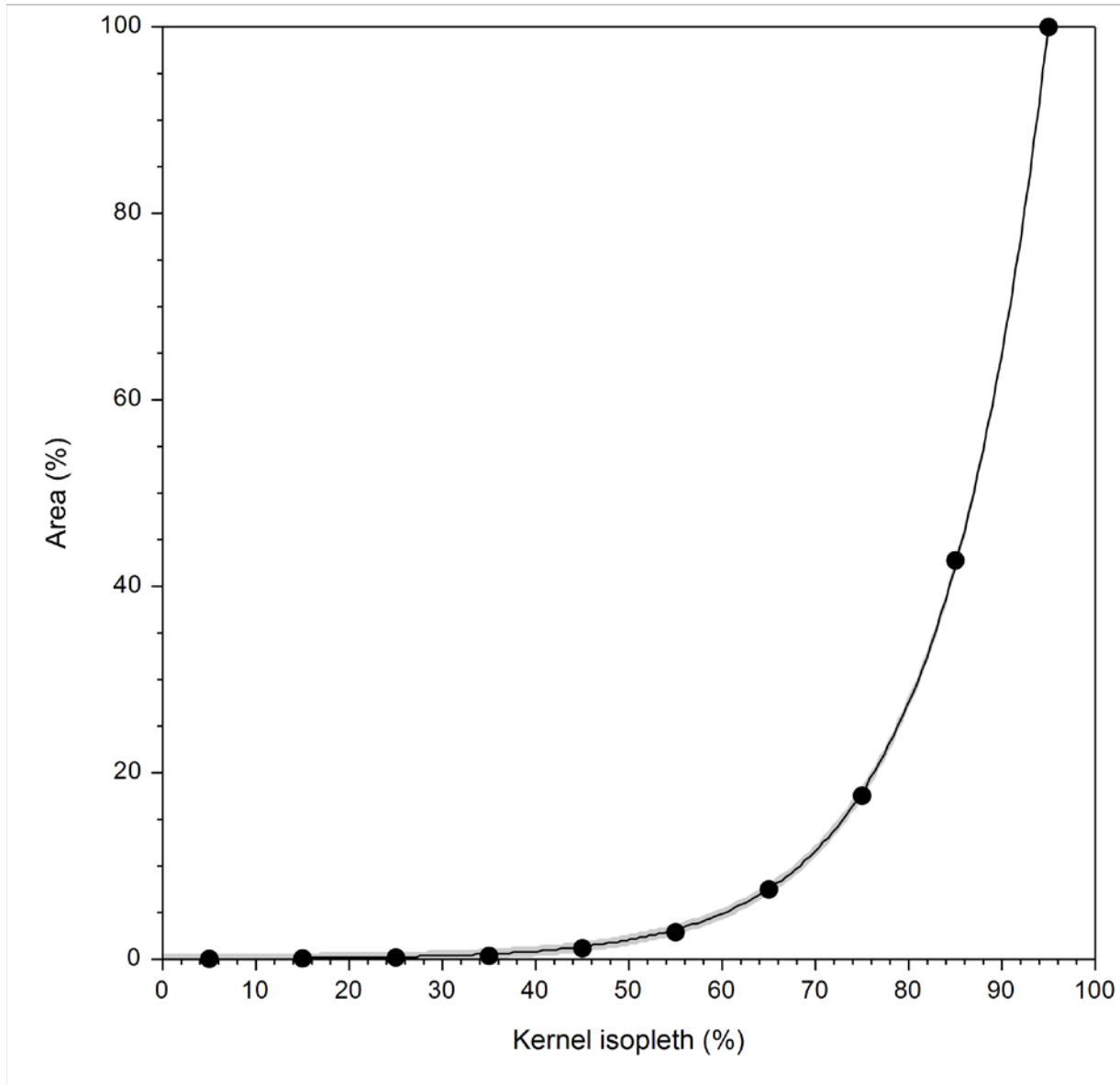
Figure 4: The Kernel isopleths (x-axis) for the crash data and the area within the isopleths (y-axis) expressed as a percentage of the area within the 95% isopleth. The function is y = 0.01033 * e^{0.08609 * x} . The shaded area around the function represents the upper and lower 95% prediction limit. Slope equals 1 at the 69.9% Kernel isopleth (11.5% of the total area within the 95% isopleth).
